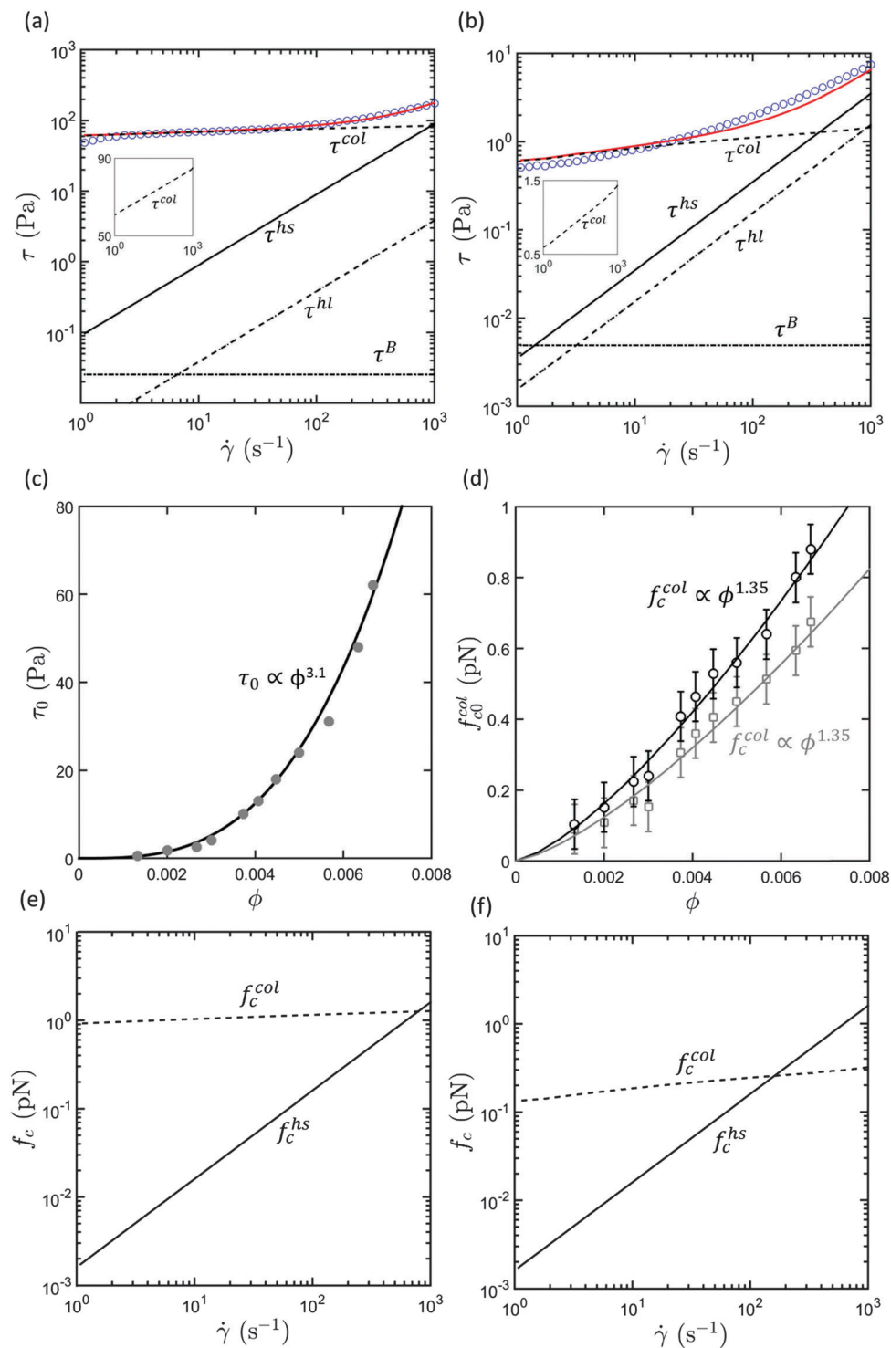
Fig. 7 (a and b) Macroscopic steady state shear stress as a function of the shear rate (curves with blue circle symbols) obtained for two TEMPO-oxidized NFC suspensions ( \phi = 0.0067 and \phi = 0.0013 ), and prediction of the micromechanical (continuous red lines). The other lines represent the contributions that are induced by the Brownian motion \tau^B , long and short hydrodynamic interactions \tau^{hl} , \tau^{hs} and colloidal interactions \tau^{col} . (c) Prediction of the dynamic yield stress \tau_0 of the micromechanical model. (d) Evolution of the characteristic colloidal force f_c^{col} as a function of the NFC content \phi for random (grey color) and orientated fibrous microstructures (black color). (e and f) Predictions of the characteristic colloidal f_c^{col} and short hydrodynamic forces f_c^{hs} as a function of \dot{\gamma} for two TEMPO-oxidized NFC suspensions ( \phi = 0.0067 and \phi = 0.0013 ).
