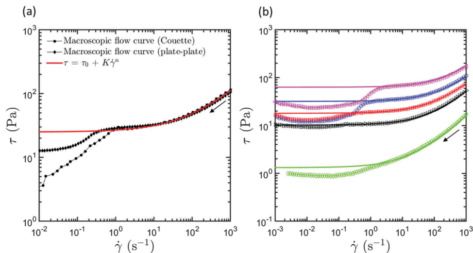
Fig. 2 (a) Flow curves obtained for a 0.85 wt% TEMPO-oxidized NFC suspension. The curve with black circle symbols represents a \tau - \dot{\gamma} curve that was obtained using a Couette rheometer by sweeping down the macroscopic shear rate \dot{\gamma} from 10^3 to 10^{-2} \text{s}^{-1} in 35 steps with times \delta t = 50 s. The curve with black diamond symbols represents a \tau - \dot{\gamma} curve obtained using a plate-plate rheometer by sweeping down the macroscopic shear rate \dot{\gamma} from 10^3 to 10^{-2} \text{s}^{-1} in 70 steps with times \delta t = 50 s. (b) Macroscopic flow curves obtained for various NFC suspensions concentrated at 0.3, 0.56, 0.7, 0.85, and 1 wt% using a plate-plate rheometer. In graphs (a) and (b), the solid lines represent the fits of the Herschel–Bulkley model (eqn (1)).
