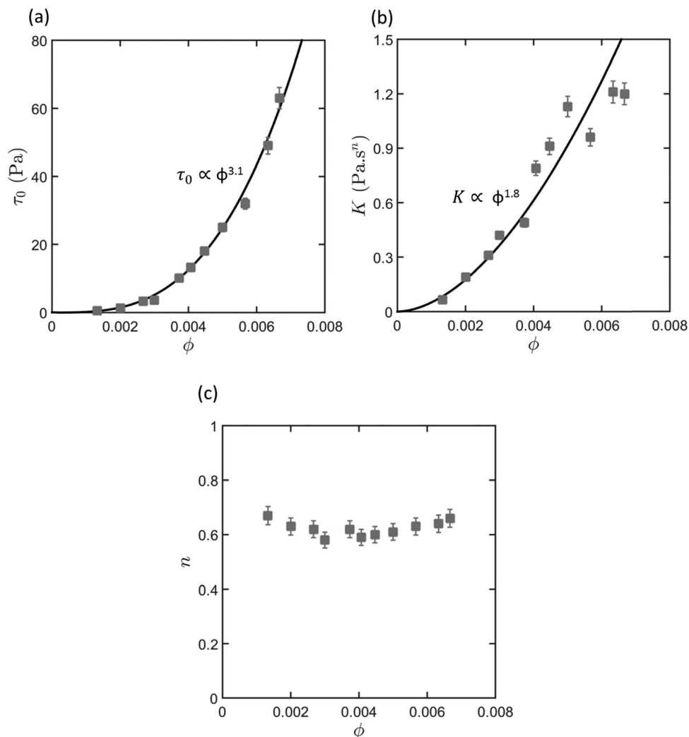
Fig. 3 Evolution of the parameters of the Herschel–Bulkley law as a function of the NFC content \phi : steady state yield stress \tau_0 (a), consistency K (b), and flow index n (c). Lines represent the power-law fits for the yield stress (a) and the consistency (b), respectively.
