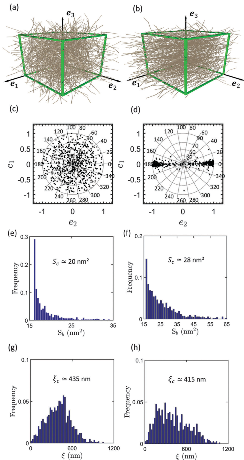
Fig. 5 Example of two idealized NFC networks for a nanofiber content \phi = 0.004 with 3D random orientation (a) and flow-induced orientation (b). For both types of microstructures, the orientation vectors \mathbf{p}_i of each tortuous NFC i were represented using a stereographic projection (pole figure of orientation) along the e_3 -direction (c and d). Typical distribution histograms of the projected bonding area S_b (e and f) and of the distance \|\xi_{ij}^0\| between the centers of mass of interacting NFCs (g and h).
