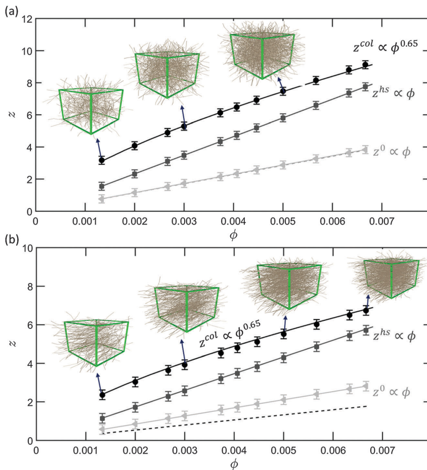
Fig. 6 Evolution of the mean coordination numbers z^z as a function of the NFC content \phi for NFC architectures with various interaction thicknesses h^z (namely h^0 = 0 , h^{hs} = d , h^{col} = 2\kappa^{-1} ), NFC waviness ( \theta_{seg} = \pi/8 ), for 3D random orientations (a) or flow-induced orientations (b). In both graphs, the dashed lines represent the evolution of the mean coordination numbers z^0 for straight NFCs ( \theta_{seg} = 0 ) and ( h^0 = 0 ).
