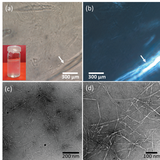
Fig. 1 Optical (a) and cross-polarized light micrographs (b) of a 0.1 wt% TEMPO-oxidized NFC suspension. The inset in (a) shows a 0.75 wt% TEMPO-oxidized NFC suspension. The white arrow indicates a partially fibrillated cellulose fiber, thus explaining the strong birefringence. (c and d) TEM micrographs of the dry suspensions after negative staining.
