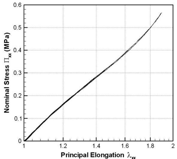
Fig. 4. Cyclic loading–unloading tensile test with increasing maximum stress: 0.1, 0.14, 0.2, 0.28, 0.4, 0.56 MPa.
