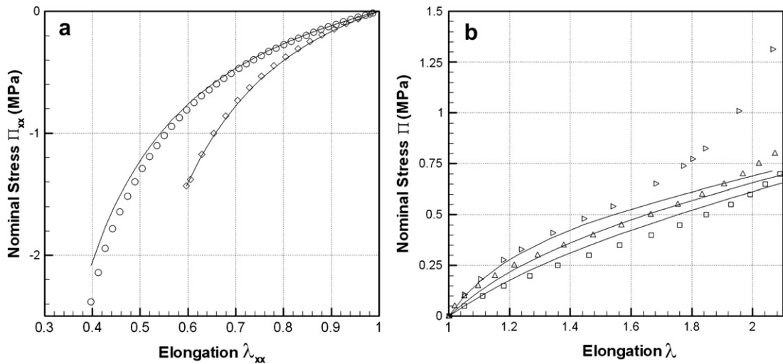
Fig. 9. Nominal stress measured and predicted by the neo-hookean model for the five tests: (□) uniaxial tensile, (△) pure shear, (○) simple compression, (◇) plane strain compression and (▷) bulge test for (a) compression tests and (b) traction tests.
