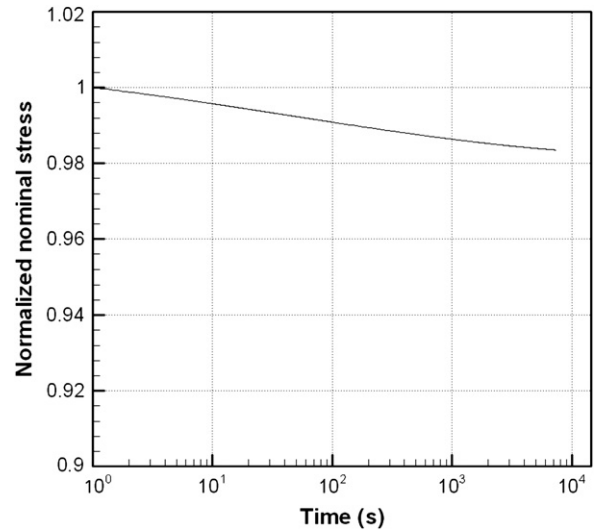
Fig. 6. Time evolution of the normalised stress \Pi_{xx}/\Pi_{xx}(t = t_0) , for a stress relaxation test recorded after a monotonic tensile test performed at \lambda=2 .
