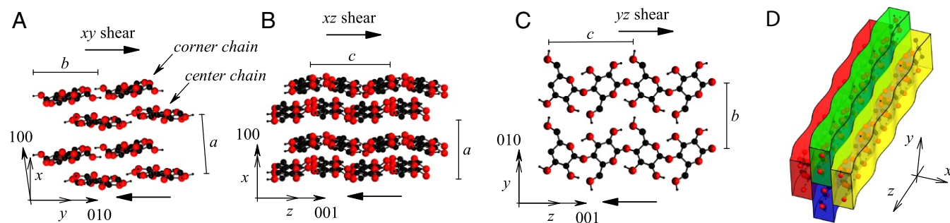
Fig. 1. Atomic structure of I_\beta cellulose. From Left to Right , molecular chains are shown in the xy ( A ), xz ( B ), and yz ( C ) planes. The direction of the applied shear strain is shown in each case. D is a 3D geometrical volume fitted on the cellulose chains to highlight their corrugation. Three-dimensional interactive representations are shown in SI Appendix, Figs. S2 and S3 . (The hydrogen atoms bonded to carbon atoms are not shown here.)
