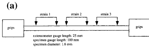
Figure 2 : (a) Schematic illustration of tensile testing using a NiTi wire and 3 local extensometers fixed, (b) time evolutions of the 3 extensometers during the tensile test plotted in Figure 1(a) [7].
