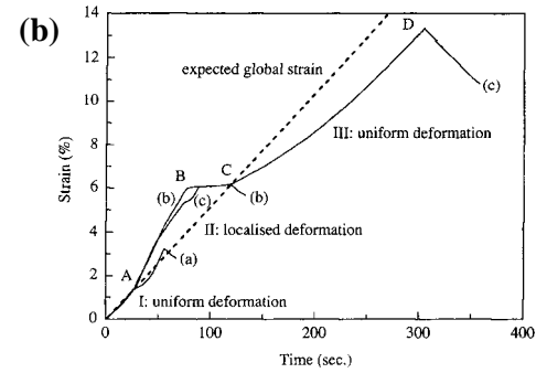
Figure 2 : (a) Schematic illustration of tensile testing using a NiTi wire and 3 local extensometers fixed, (b) time evolutions of the 3 extensometers during the tensile test plotted in Figure 1(a) [7].
