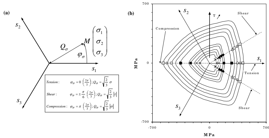
Figure 8 : (a) Polar representation of the stress tensor in the deviatoric stress plane, (b) experimental shear, tension and compression results obtained on a superelastic NiTi polycrystal at different temperatures above M_s and identification of the yield criterion (5) proposed in [14] ( \gamma_0 = 0.9 and n_o = 0.1 ).
