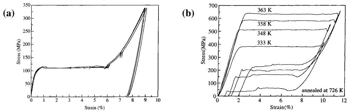
Figure 1: Tensile stress-strain curves obtained with NiTi polycrystals (a) in ferroelasticity [7] ;(b) in superelasticity [10].
