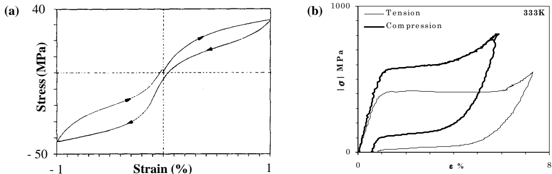
Figure 3 : Cyclic tension-compression superelastic test on one CuZnAl polycrystalline sample [19], (b) monotonic tension and compression superelastic tests on two NiTi polycrystalline samples [14].
