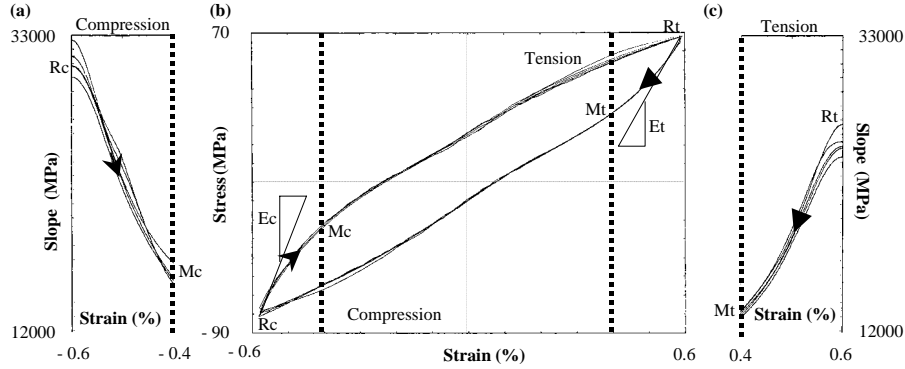
Figure 4 : Cyclic tension-compression test on a CuZnAl polycrystal : (b) stress-strain curve, (a) slope during unloading in compression, (c) slope during unloading in tension [17].
