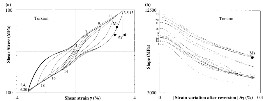
Figure 6 : Cyclic torsion test with subloops on the same CuZnAl polycrystal as that shown in Figure 4 [17], (a) stress-strain curve, (b) slope modulus during unloading after reversion (all subloops).
