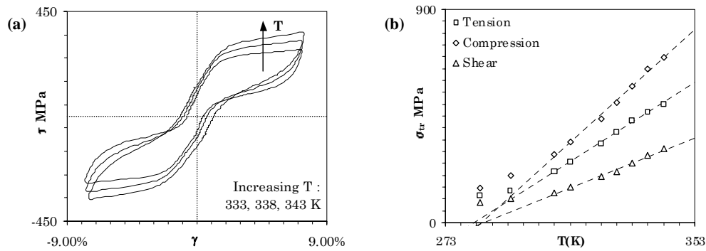
Figure 5 : (a) Cyclic superelastic shear tests performed at different temperatures on a NiTi polycrystal, (b) temperature dependence of the threshold stress to induce martensite for the same alloy in tension, compression and shear [14].
